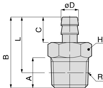
Taper pipe thread
