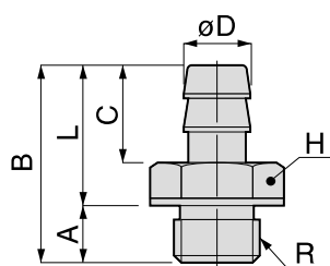
Metric thread
