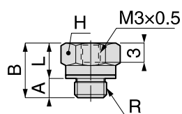
Metric thread type
