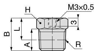
Taper pipe thread type
