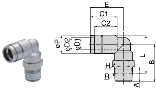
Taper pipe thread type
